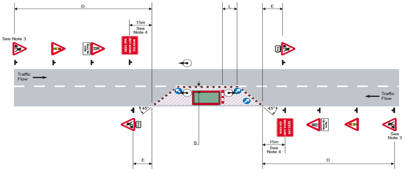
Traffic control by portable traffic signals
